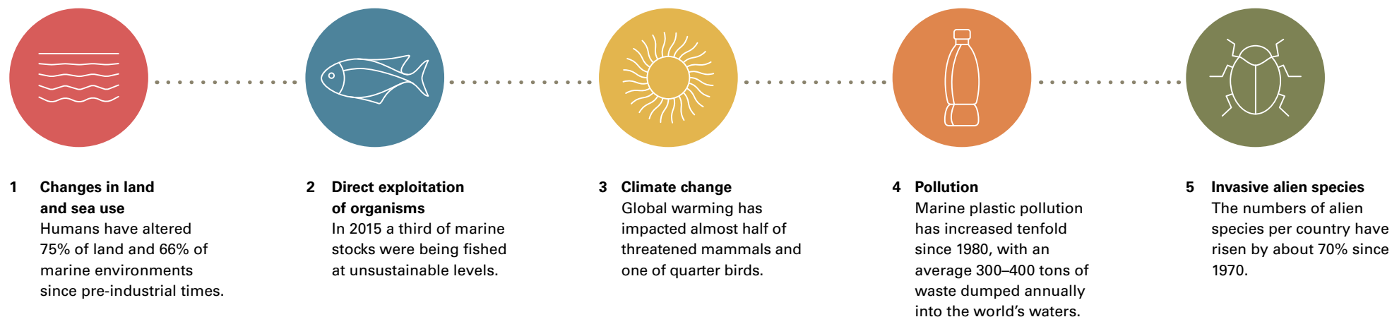
Fig. 3 Five main drivers of biodiversity loss
